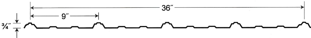
Sandstone
